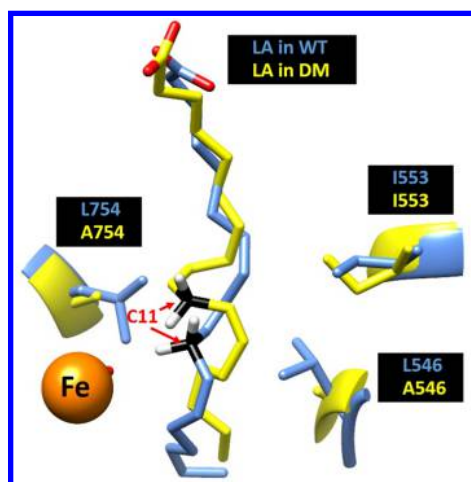
Figure 6. Comparison between the ground state substrate binding mode in WT (blue) and DM (yellow). The reactive carbon C11 is colored as black, iron colored as orange.
