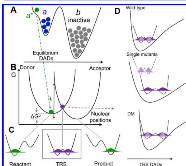
Figure 5. Rate constants for enzyme catalyzed nonadiabatic hydrogen transfer can be formalized as k_{\text{obs}} = K_{\text{eq}} \cdot k_{\text{PCET}} . 9,28,30 (A) K_{\text{eq}} ( \ll 1 ) represents a stochastic ground state search through inactive conformations ( b ) to reach catalytically active E-S complexes ( a conformer). Subsequent thermal sampling further reduces the distance between the H-donor and acceptor as seen in the pretunneling a^* conformer. (B–D) illustrate contributions from k_{\text{PCET}} : (B) Heavy atom protein motions produce transiently degenerate energies for the reactant and product wells, a prerequisite for wave function overlap at the tunneling ready state (TRS) (C). (D) The effective potential along the DAD sampling coordinate varies, starting with \Delta E_{\text{a}} \approx 0 for native enzyme (top), becoming \Delta E_{\text{a}} \gg 0 when the DAD is elongated following single mutations (middle) and finally arriving at the catastrophic DM scenario in which the DAD is elongated, but coupled with a rigid DAD sampling potential (bottom). In panel D, light purple refers to the shorter wave function distribution for deuterium, and dark purple represents the more distributive protium wave function.
